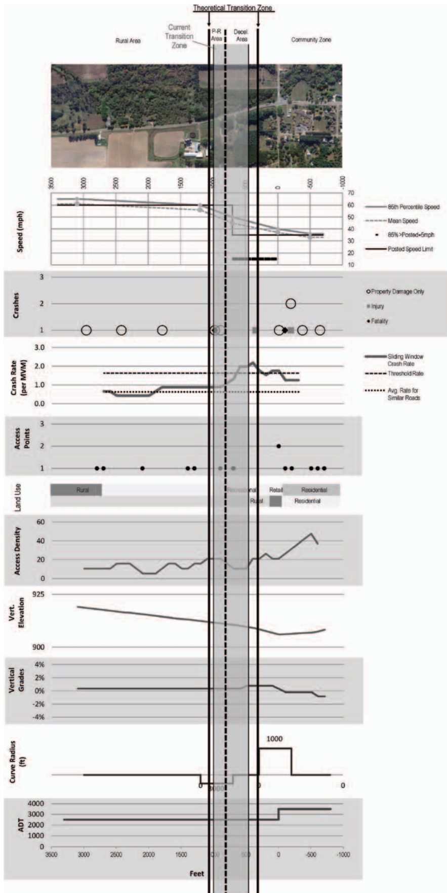
Figure 4-2. Straight-line diagram tool (P-R = perception-reaction, Decel = deceleration, Vert. = vertical).
