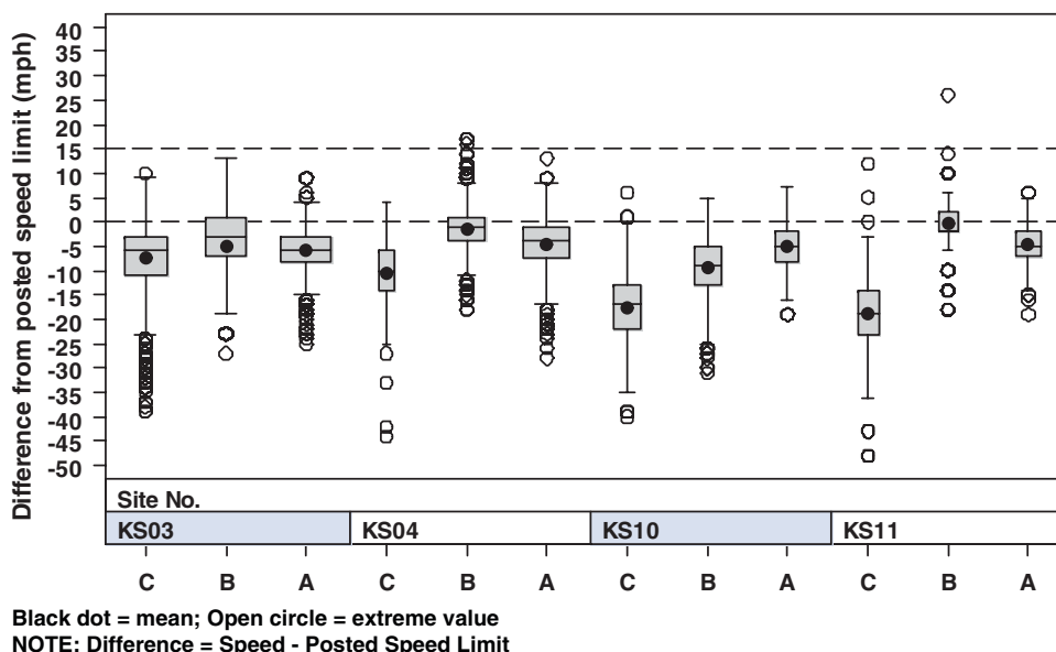
Figure 3-6. Speed differences from posted speed limit—welcome signs.
