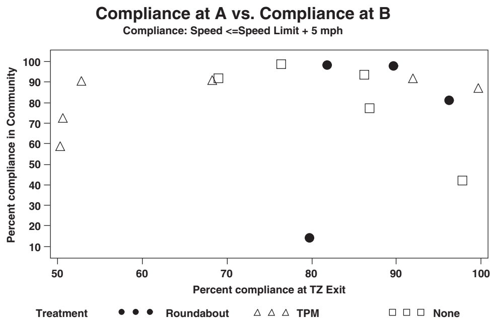
Figure 3-11. Observed community (Location A) compliance versus exit (Location B) compliance—posted speed limit + 5 mph criterion.
