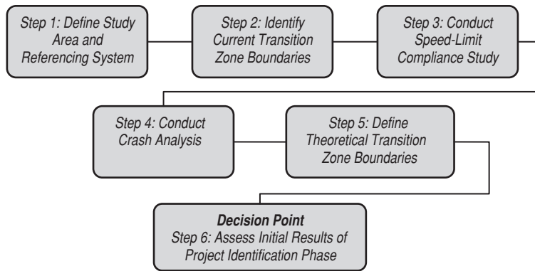
Figure 4-3. Recommended steps of project identification phase.
