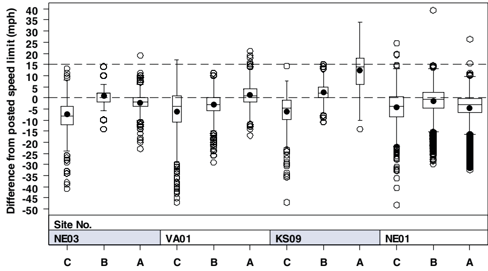
Figure 3-4. Speed differences from posted speed limit—roundabouts.
