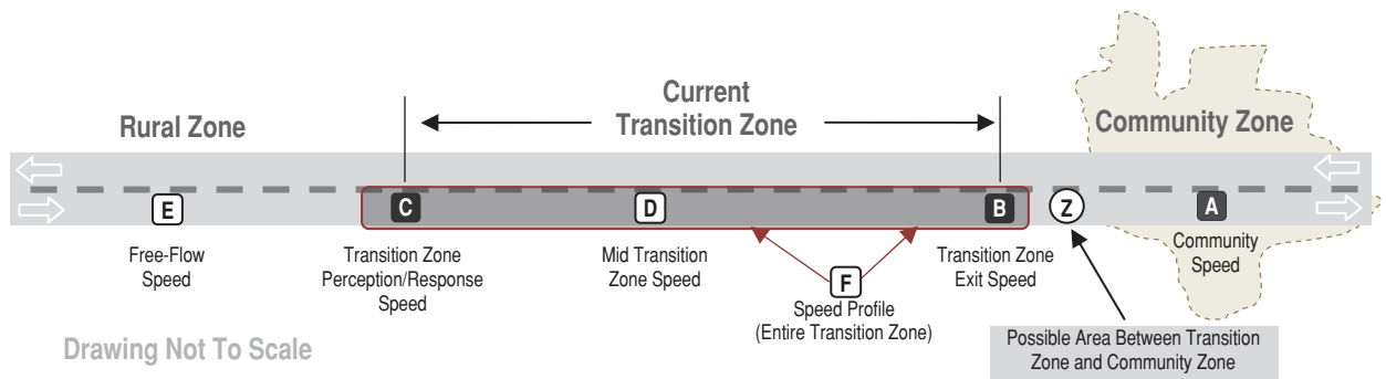
Figure 4-4. Speed data collection locations within the study area.
