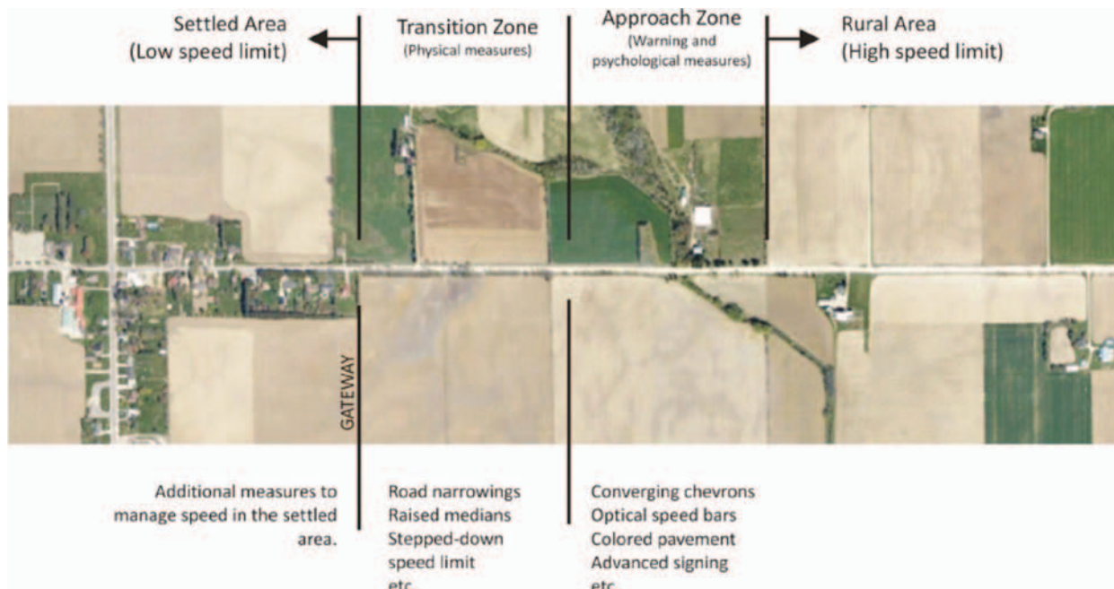
Figure 2-1. Transition zone and approach zone concepts (Forbes, 2011).
