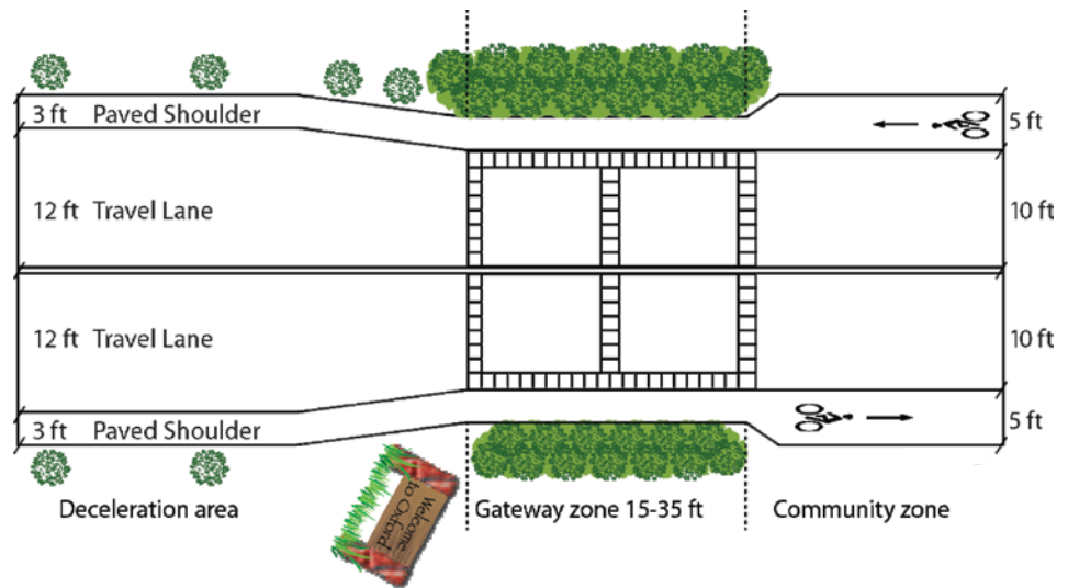
Figure 4-16. Rendering of a gateway.
