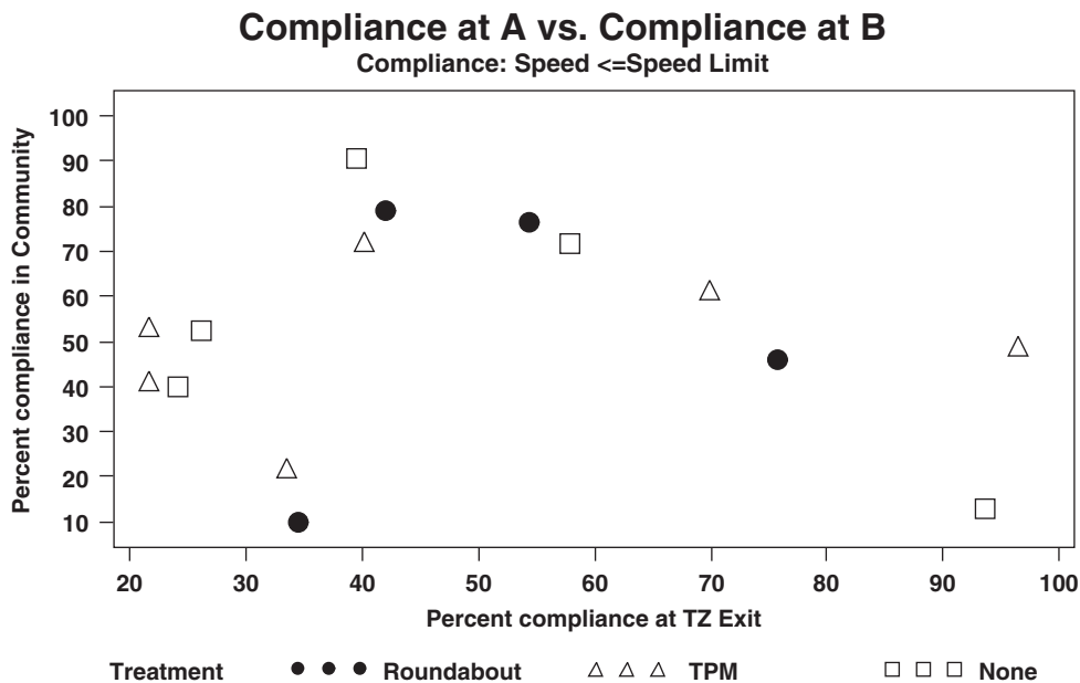
Figure 3-10. Observed community (Location A) compliance versus exit (Location B) compliance—posted speed limit criterion.
