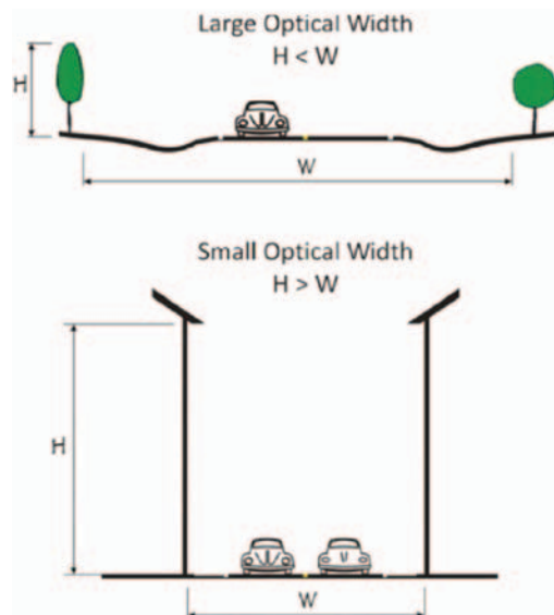
Figure 4-17. Relationship between horizontal elements and vertical dimensions (Forbes, 2011).
