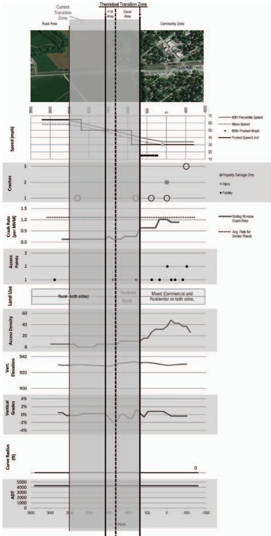
Figure 4-18. Straight-line diagram for example study site.
