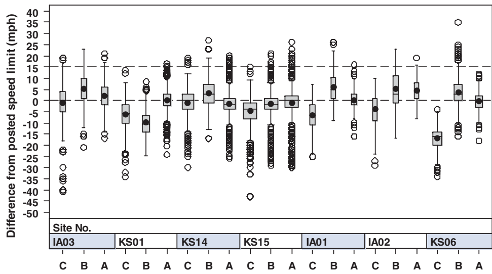
Figure 3-5. Speed differences from posted speed limit—TPMs.
