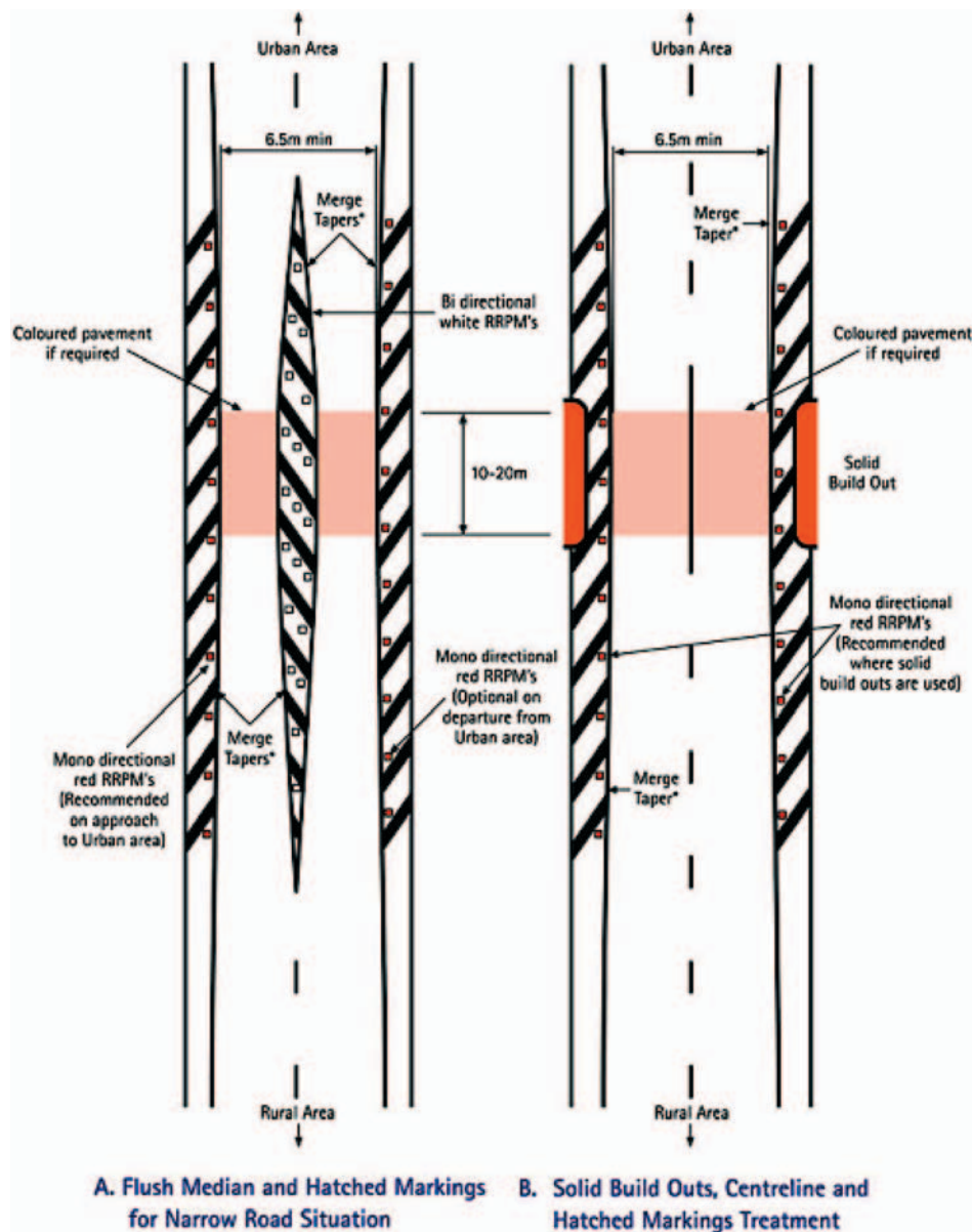
Figure 2-7. Pavement markings and RRPMs without solid islands (RRPM = retroreflective pavement markings) (LTSA, 2002).
