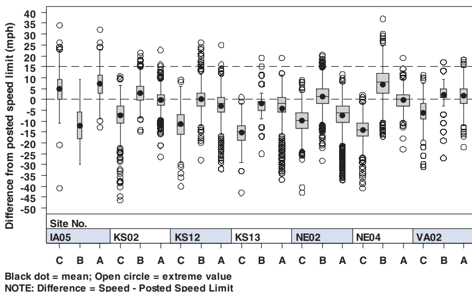
Figure 3-7. Speed differences from posted speed limit—no treatment.
