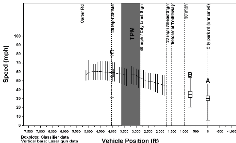
Figure 3-3. Vehicle speed profile example.
