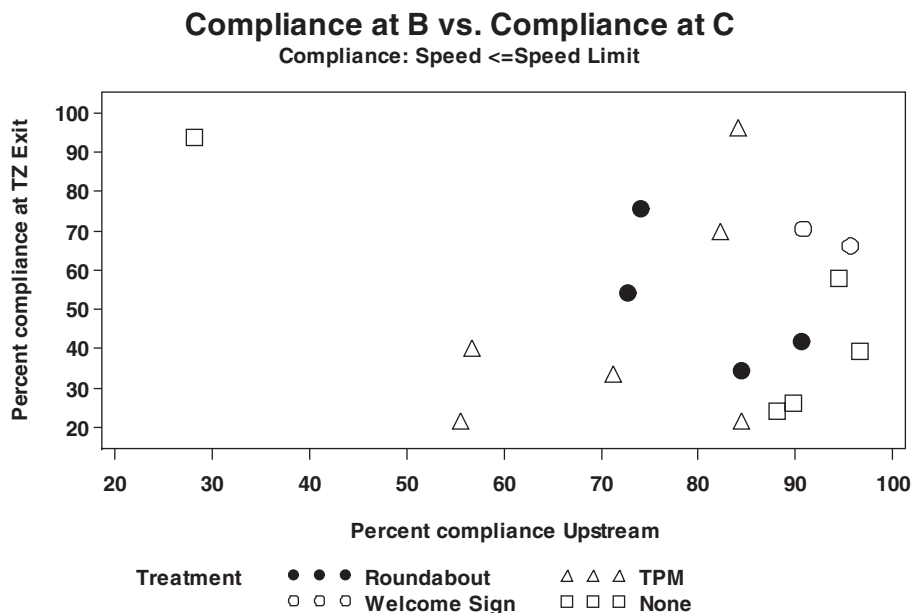
Figure 3-8. Observed exit (Location B) compliance versus upstream (Location C) compliance—posted speed limit criterion (TZ = transition zone).
