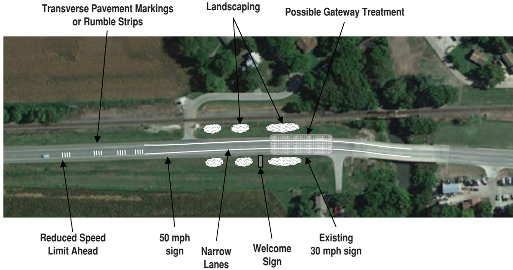
Figure 4-19. Suggested transition zone treatments to consider at example study site.
