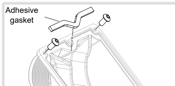
Side of Pole
