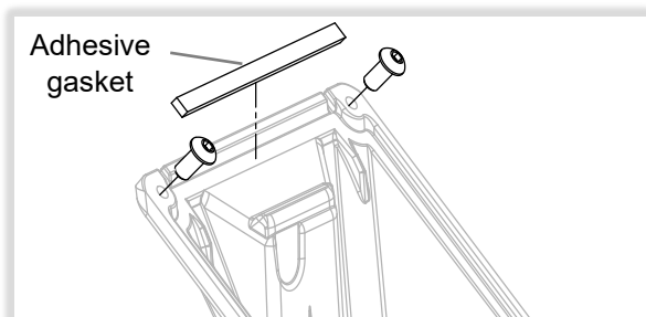
Top of Pole
