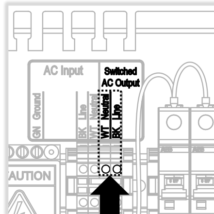
MX 400 connections for AC fixtures
